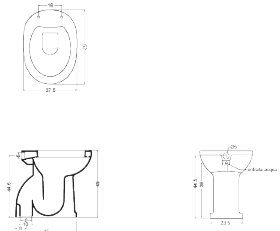
Cod. AGVB102 WC-bidet a terra scarico pavimento / Back to wall WC-bidet, floor drain
