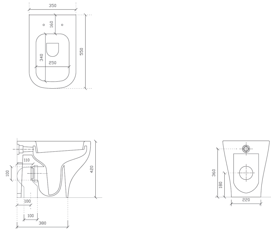
Cod. LOVATSQ WC a terra / Back to wall WC
