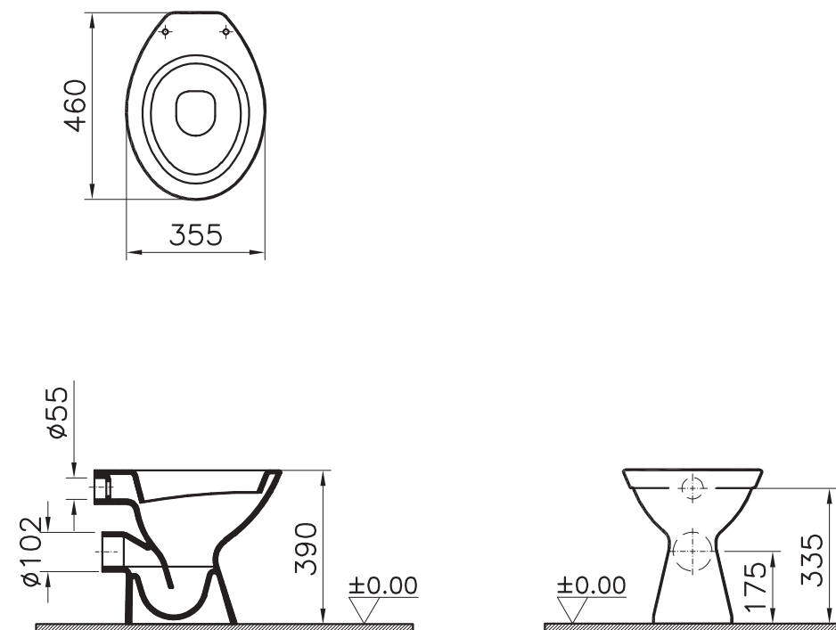
Cod. 6858L003-0101 WC a terra scarico parete / Back to wall WC, wall drain
