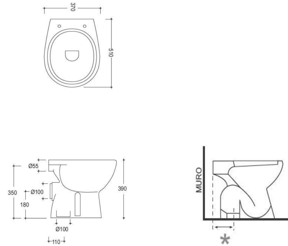
Cod. 00204 WC a terra, scarico parete / Back to wall WC, wall drain
