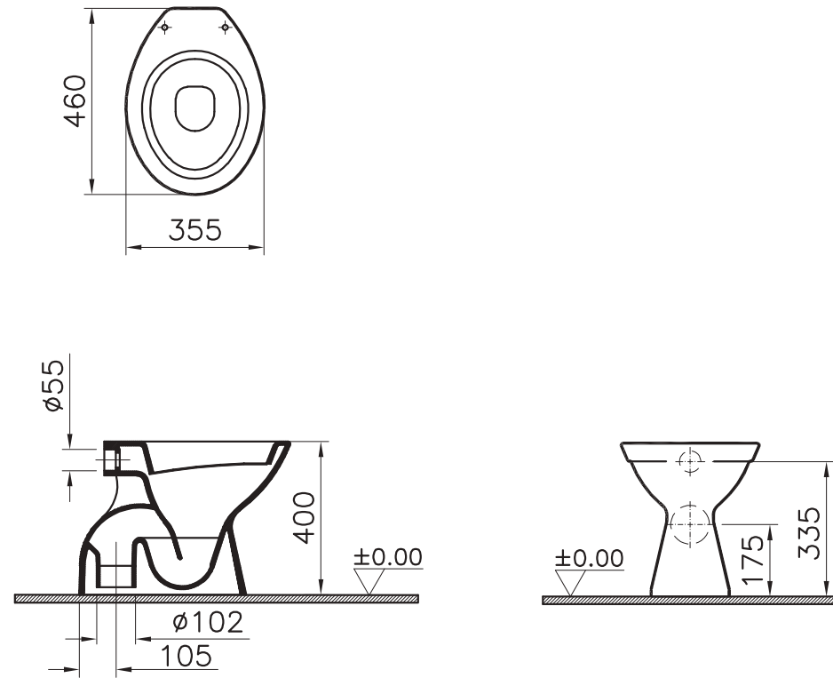
Cod. 6858L003-0101 WC a terra scarico parete / Back to wall WC, wall drain
