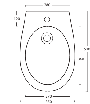
Cod. W0202 Bidet a terra / Back to wall bidet
