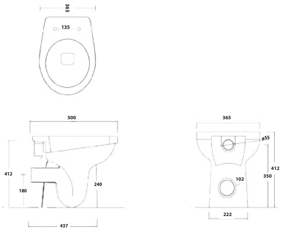
Cod. BEVA102 WC a terra, scarico parete / Back to wall WC, wall drain
