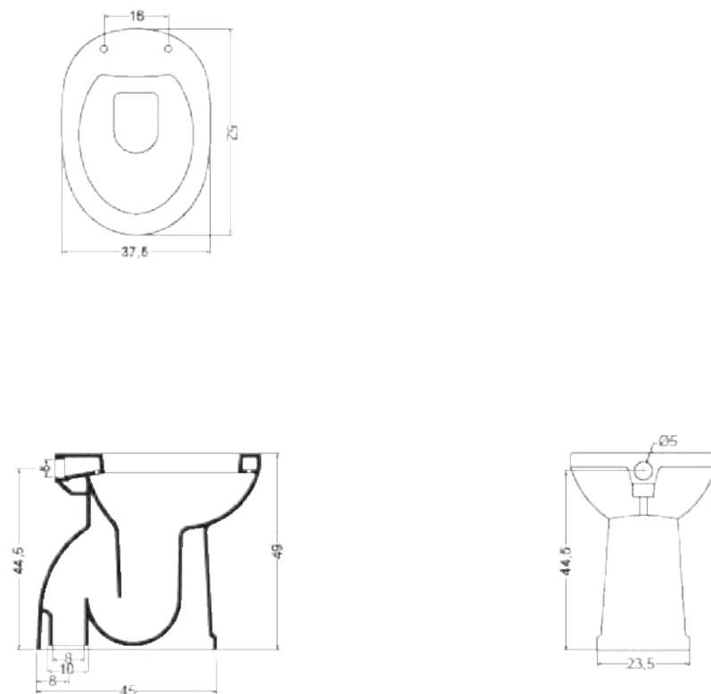
Cod. AGVA100 WC a terra scarico pavimento / Back to wall WC, floor drain
