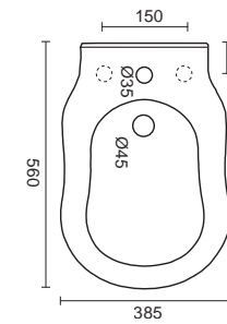
Cod. 3060 Bidet a terra / Back to wall bidet
