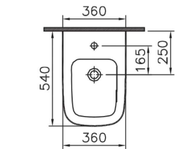
Cod. 5509L003-0288 Bidet a terra / Back to wall bidet
