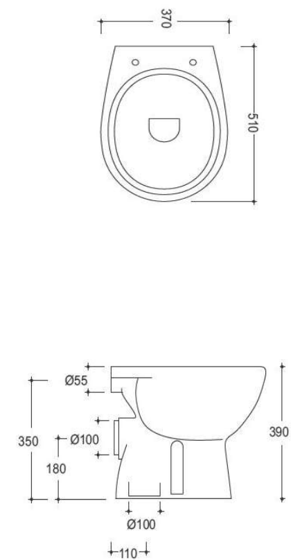
Cod. 00204 WC a terra, scarico parete / Back to wall WC, wall drain
