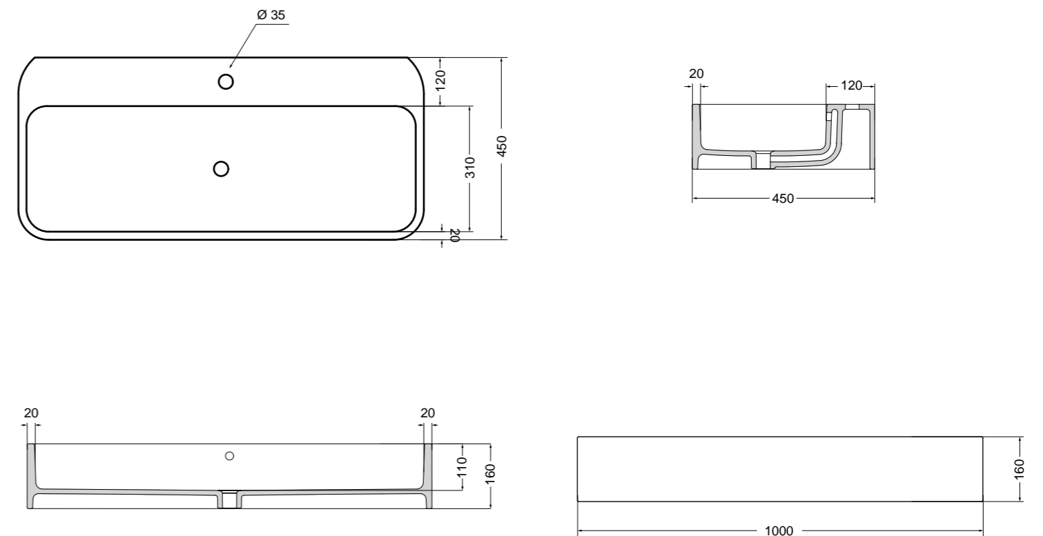
86400 lavabo appoggio/sospeso 100x45 cm_counter-top/wall-hung basin 100x45 cm
