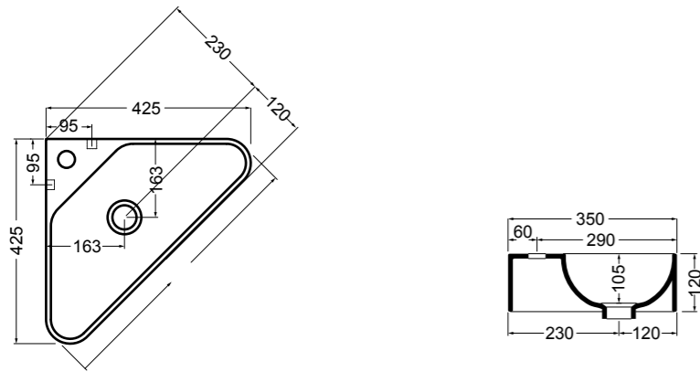
WS107 NORMAL lavabo da appoggio 42 cm_NORMAL counter-top basin 42 cm WS115 NORMAL lavabo sospeso 42 cm_NORMAL wall hung basin 42 cm
