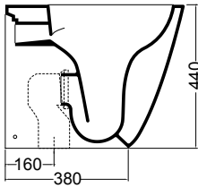
160 mm con curva tecnica Art. AF0002 with technical curve Art. AF0002
