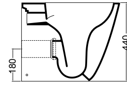
Raccordo a parete Art. AF0011 Wall connection Art. AF0011
