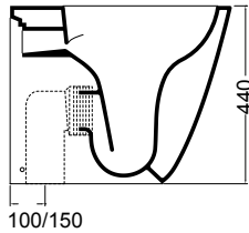
max 150 mm min. 100 mm con curva tecnica Art. AF0004 with technical curve Art. AF0004
