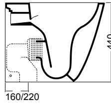
max 220 mm min. 160 mm con curva tecnica Art. AF0003 with technical curve Art. AF0003
