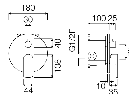
HKINC143C Incasso doccia tondo Recessed round shower control
