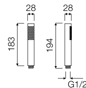
HKDOC131C Doccetta tonda Round handheld showerhead
