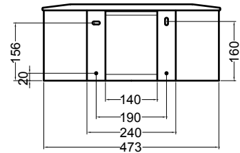
VISTA POSTERIORE REAR VIEW
